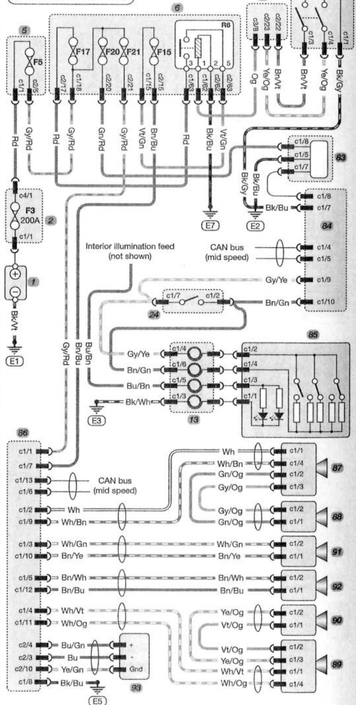
Typical audio system (with keyless system)
